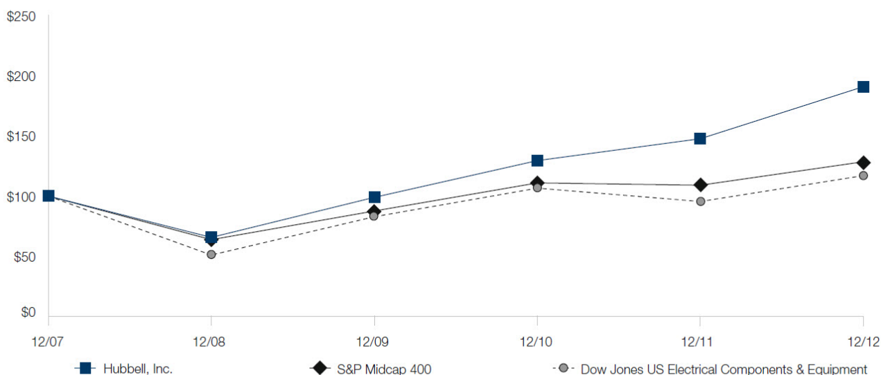
COMPARISON OF 5 YEAR CUMULATIVE TOTAL RETURN* Among Hubbell, Inc., the S&P Midcap 400 Index, and The Dow Jones US Electrical Components & Equipment Index
